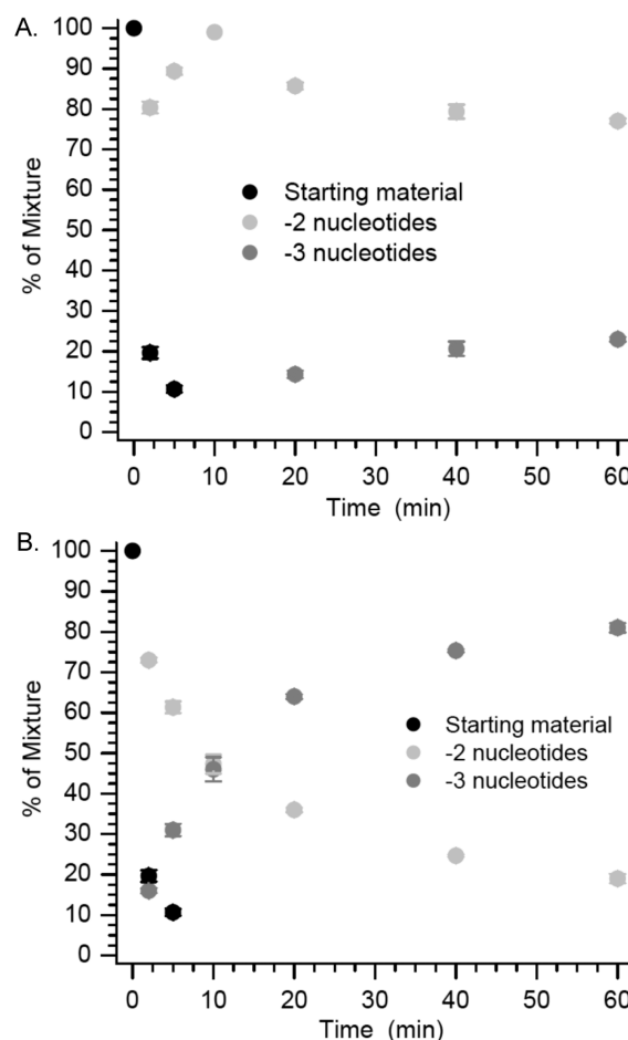
Figure 3. FEN1 incision of F ( 3' - ^{32} P-5): (A) 1 nM FEN1; (B) 10 nM FEN1.
