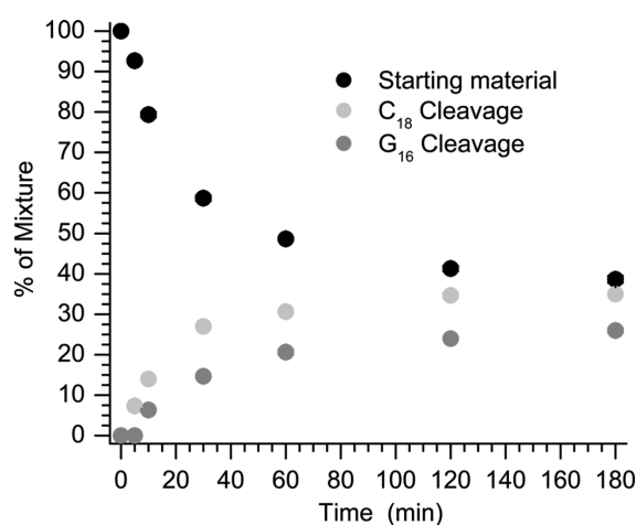
Figure 4. Incision of ternary complex containing T-al ( 5' - ^{32} P-8) by UvrABC.
