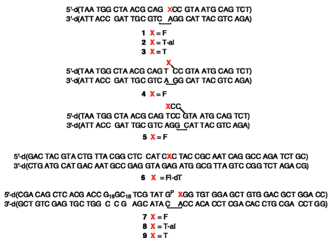
Chart 1. Nucleic Acid Complexes Used in This Study
