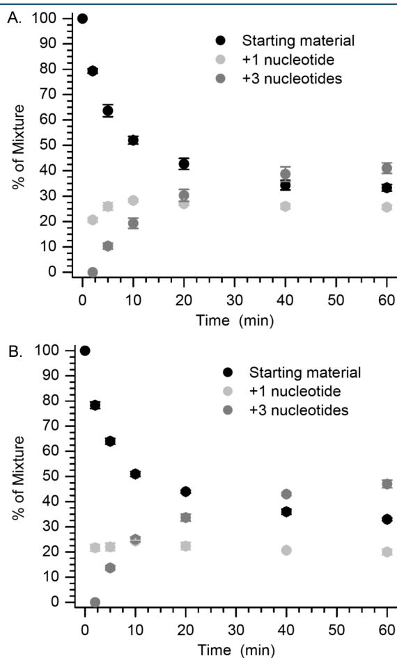
Figure 1. Strand displacement synthesis of T-al (5'- 32 P-2) by Pol \beta (1 nM) in the presence of (A) 1 nM FEN1 and (B) 10 nM FEN1.
