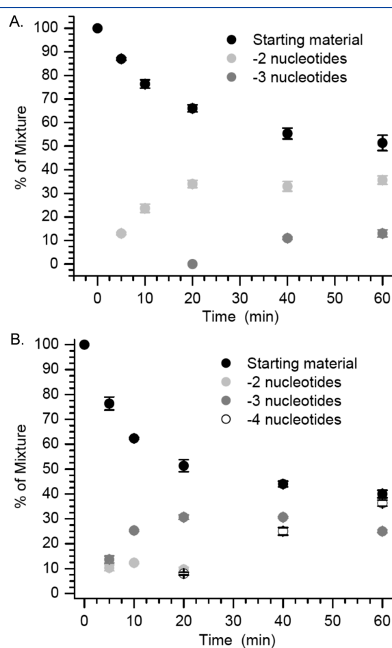
Figure 2. Cleavage of T-al (3'- 32 P-2) in the presence of Pol \beta (1 nM) and (A) 1 nM FEN1 and (B) 10 nM FEN1.
