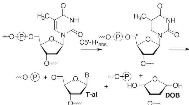
Scheme 1. Formation of T-al and DOB from a C5'-Radical
