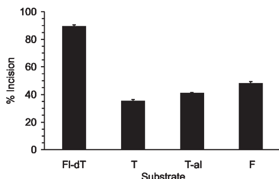
Figure 5. Comparison of UvrABC incision of DNA containing FI-dT (6), thymidine (9), T-al (8), and F (7) in 30 min.
